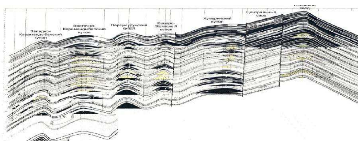
Figure 2. Southern Mangyshlak. Event chart. [1]
