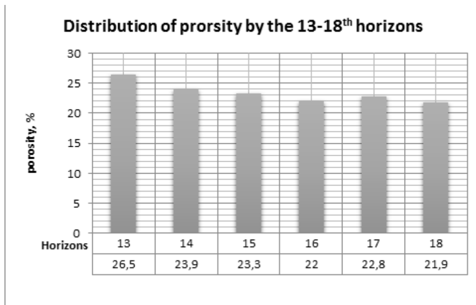
Figure 5. Distribution of average porosity by the horizons
