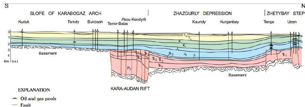
Figure 1. Geological profile. South Mangyshlak. [1]
