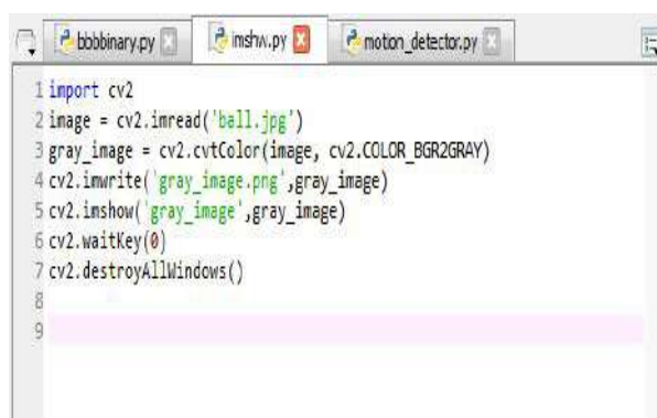
Figure 1. The pseudo-code in python
