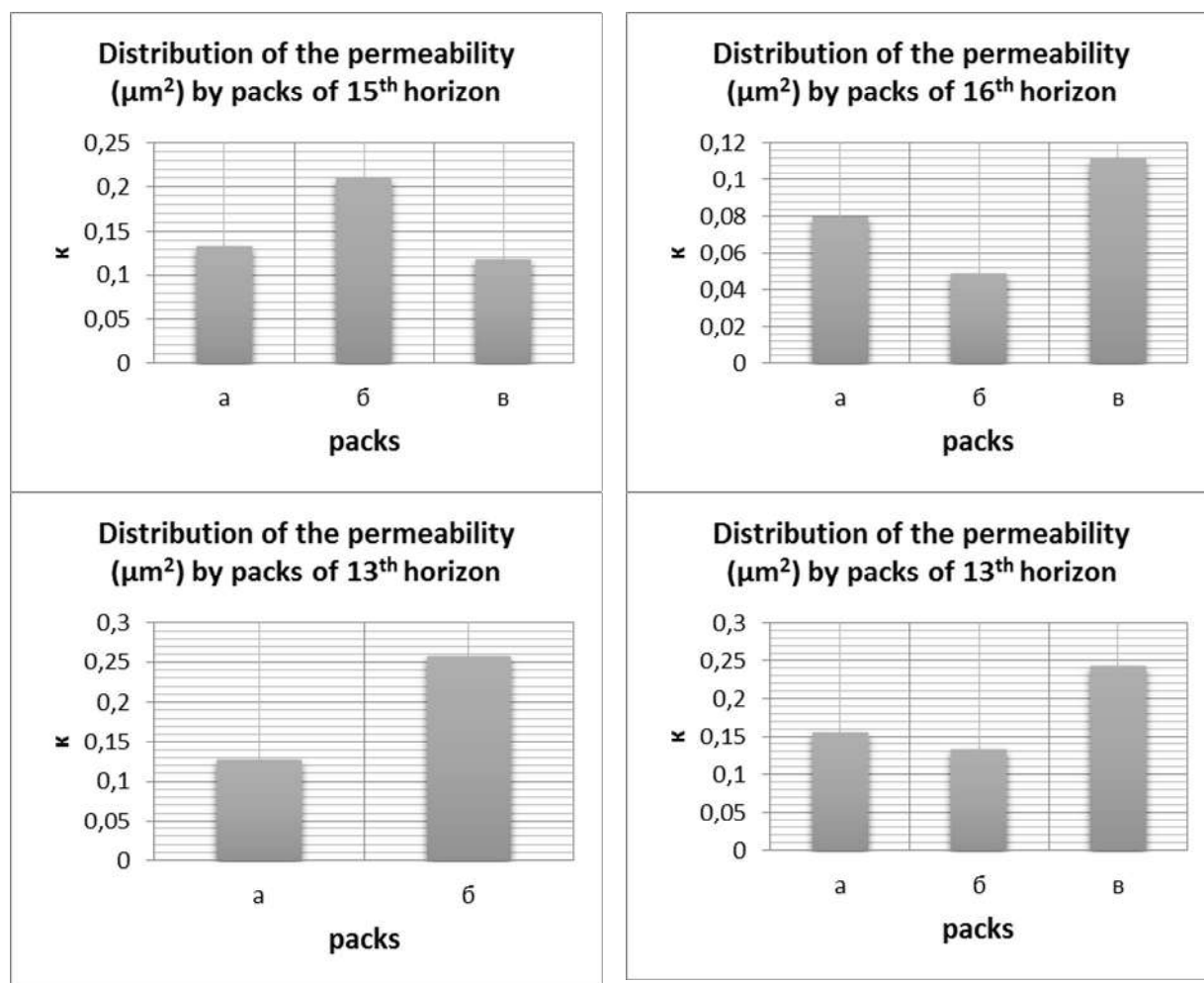
Figure 6. Distribution of permeability horizons
