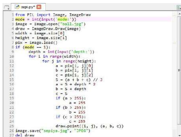
Figure 3. The pseudo-code in python
